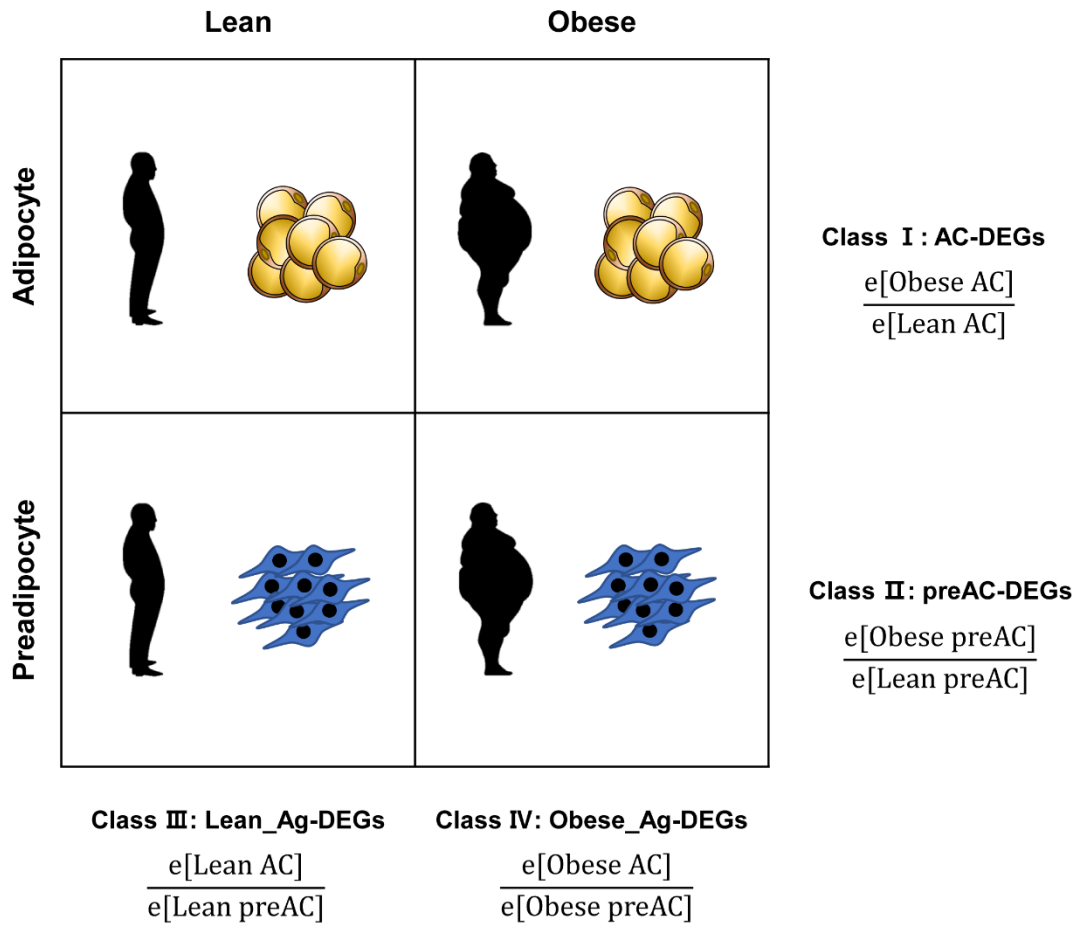
Figure S1. Schematic of identification of four different classes of DEGs.
